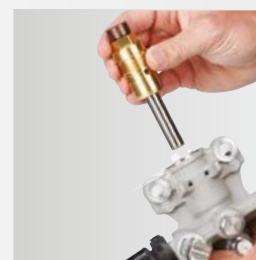
4. Install new cartridge and replace pump
